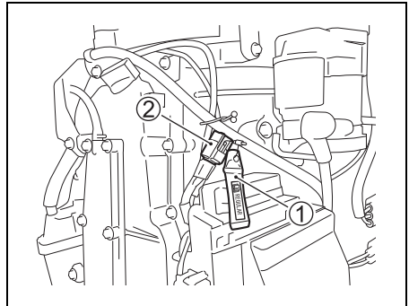
Regular rotation lower unit
